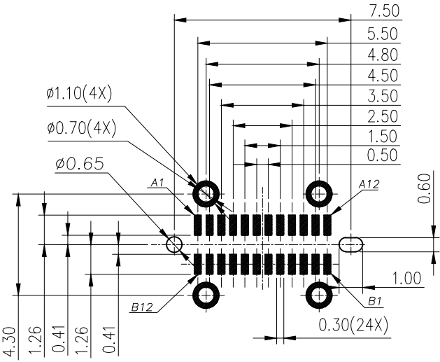
RECOMMENDED PCB LAYOUT(TOP VIEW) THICKNESS 1.0±0.10MM;DEFAULT TOLERANCE:±0.05
