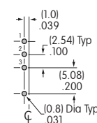
V1 Terminals
