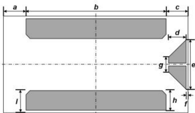
底视图/Bottom View
