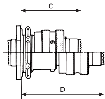
Jam nut receptacle (type 7) with plug (type 5)
