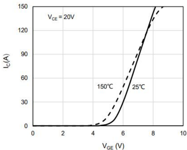
Fig.6 Transfer characteristics
