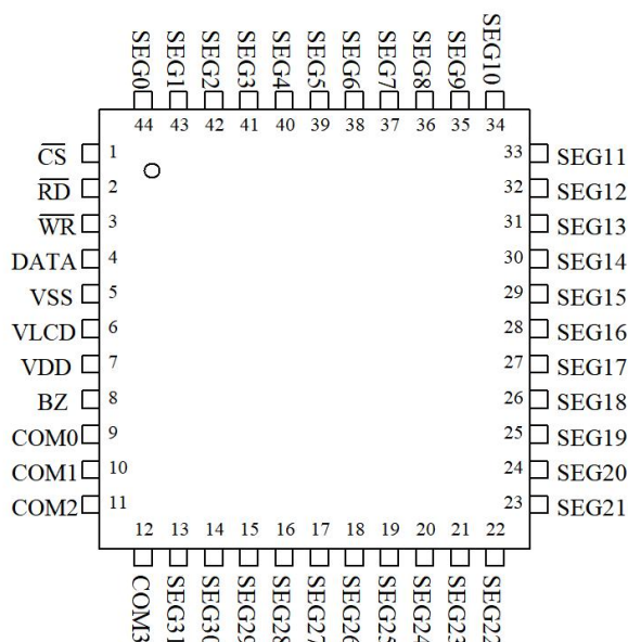
HT1621B LQFP-44
