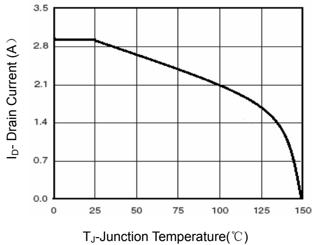
Figure 4 Drain Current
