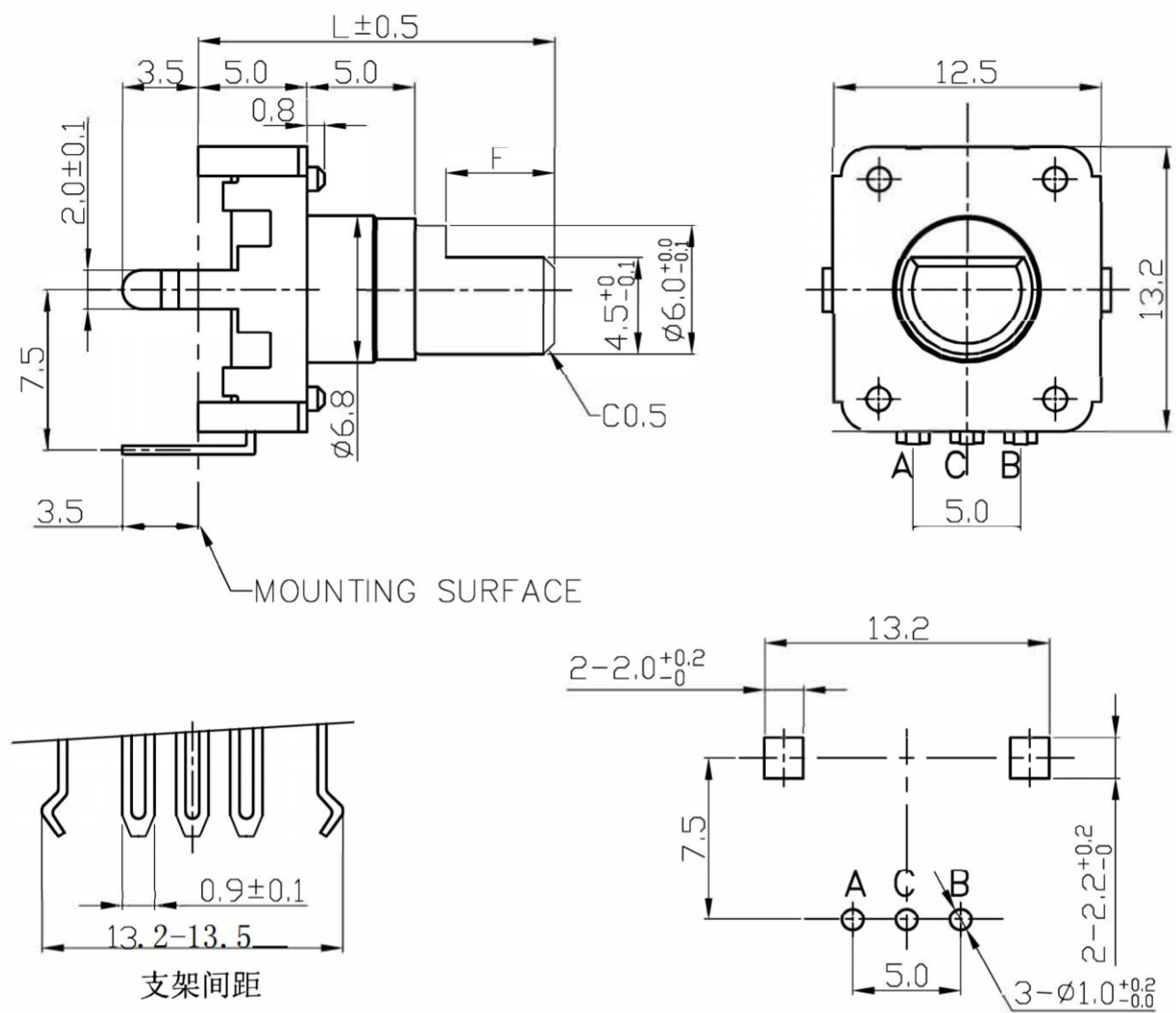
P.C.B MOUNTING HOLE DETAIL
