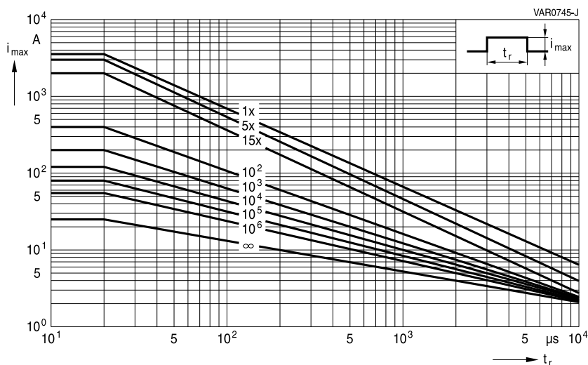
SIOV-S10K510 ... K680E2K1
