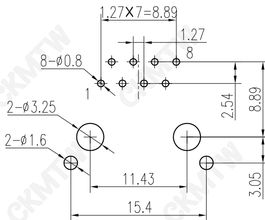
PCB LAYOUT
