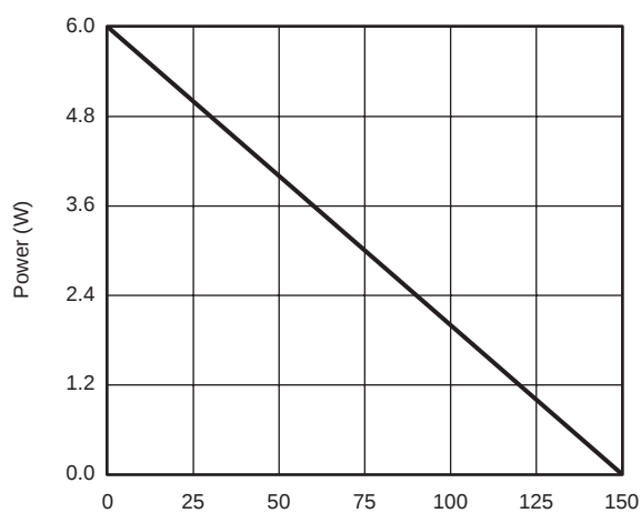
Power, Junction-to-Ambient
