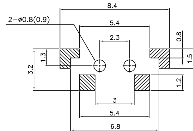
PCB. 焊接图 PCB. WELDING DRAWING
