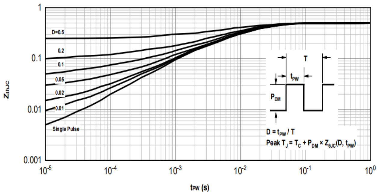
Fig.15 Transient thermal impedance from junction to case
