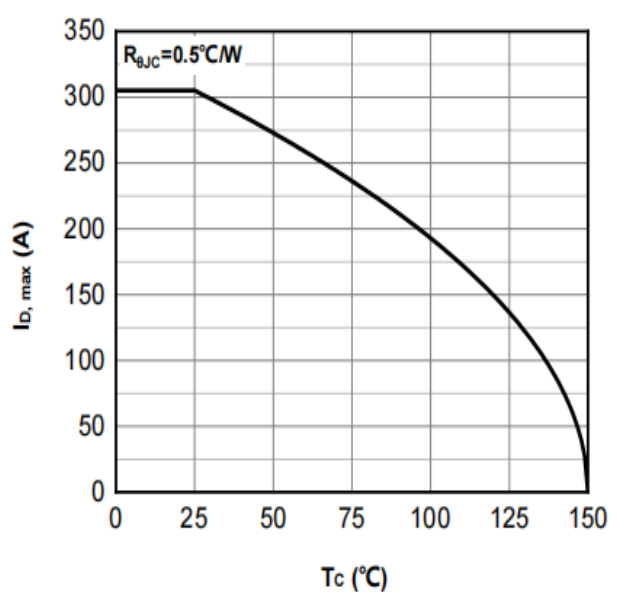
Fig.12 Max. continuous drain current vs case temperature
