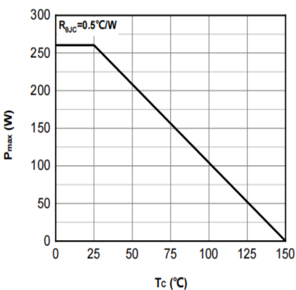
Fig.11 Max. power dissipation vs case temperature
