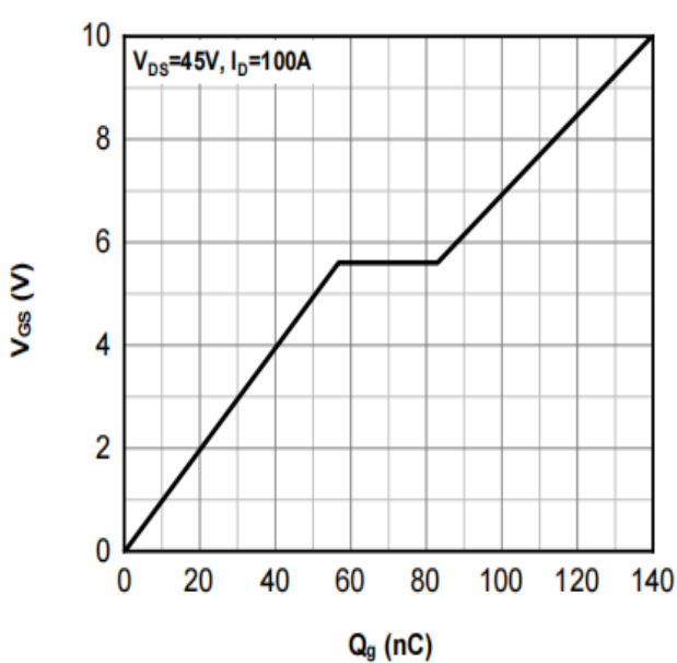
Fig.6 Typ. gate charge
