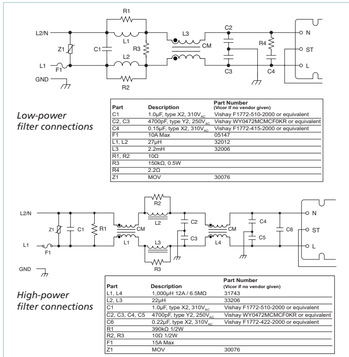
Figure 13 — Filter connections
