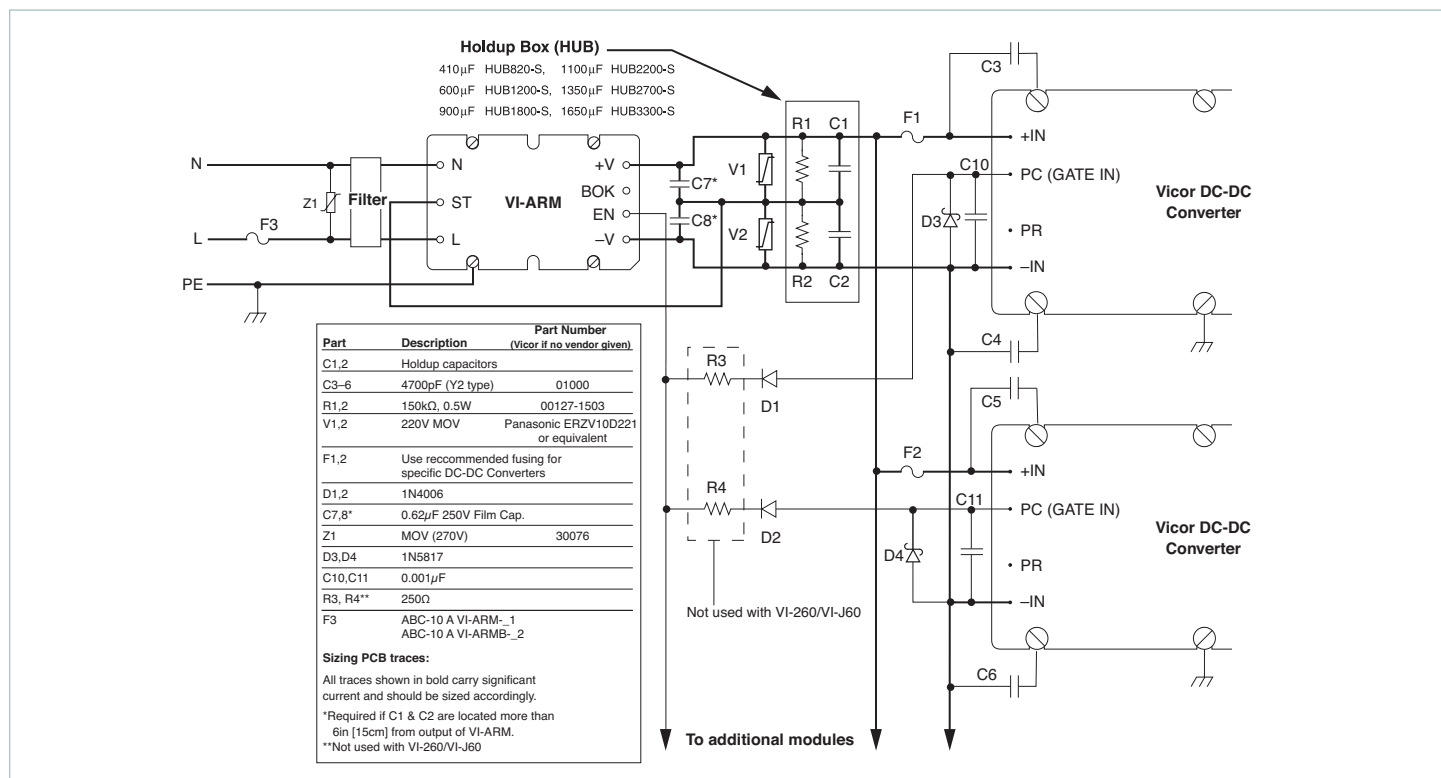
Figure 10 — Converter connections
