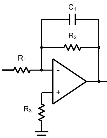
Figure 5. Low Pass Active Filter
