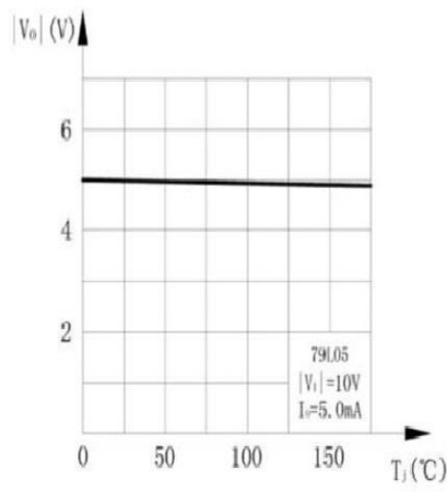
The curve of the output voltage and junction temperature
