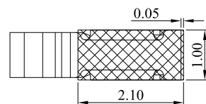
RECOMMENDED PCB LAYOUT TOLERANCE:±0.05MM (FOR REFERENCE ONLY)
