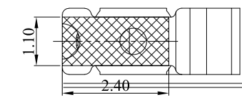
RECOMMENDED PCB LAYOUT TOLERANCE: ±0.05MM (FOR REFERENCE ONLY)
