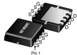
DFN3X3-8L (TSDSON-8(3.3x3.3))
