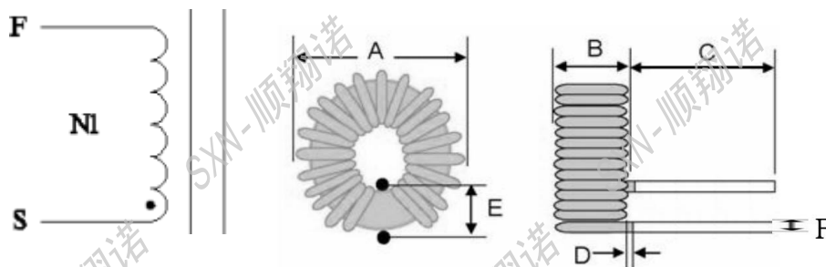
SCHEMATIC
