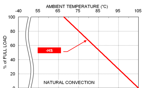
RHD40-110S05W Derating Curve With Heat-sink
