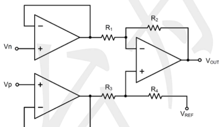
Figure 5. Instrumentation Amplifier
