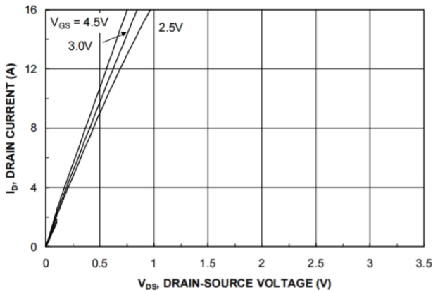
Figure 1. On-Region Characteristics.
