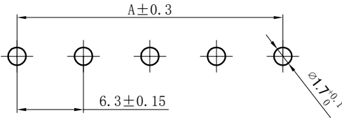
PCB LAYOUT
