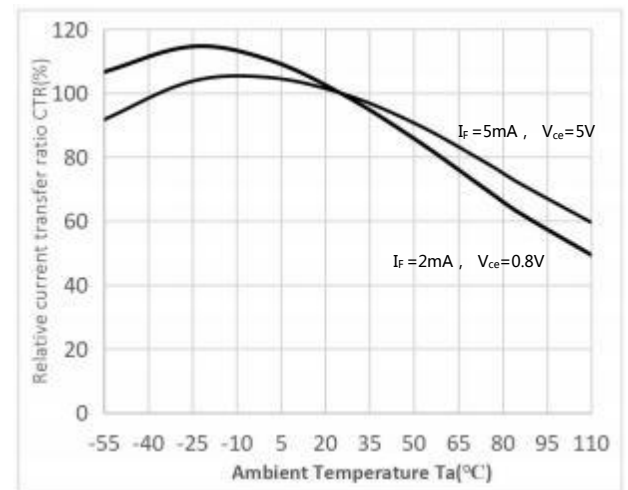
Fig.6 Relative Current Transfer Ratio vs. Ambient Temperature
