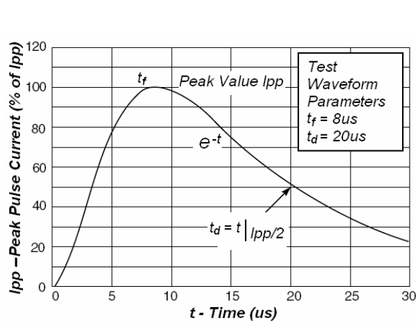
Fig2. Pulse Waveform
