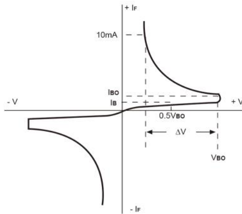
DIAGRAM 1: CURRENT-VOLTAGE CHARACTERISTICS
