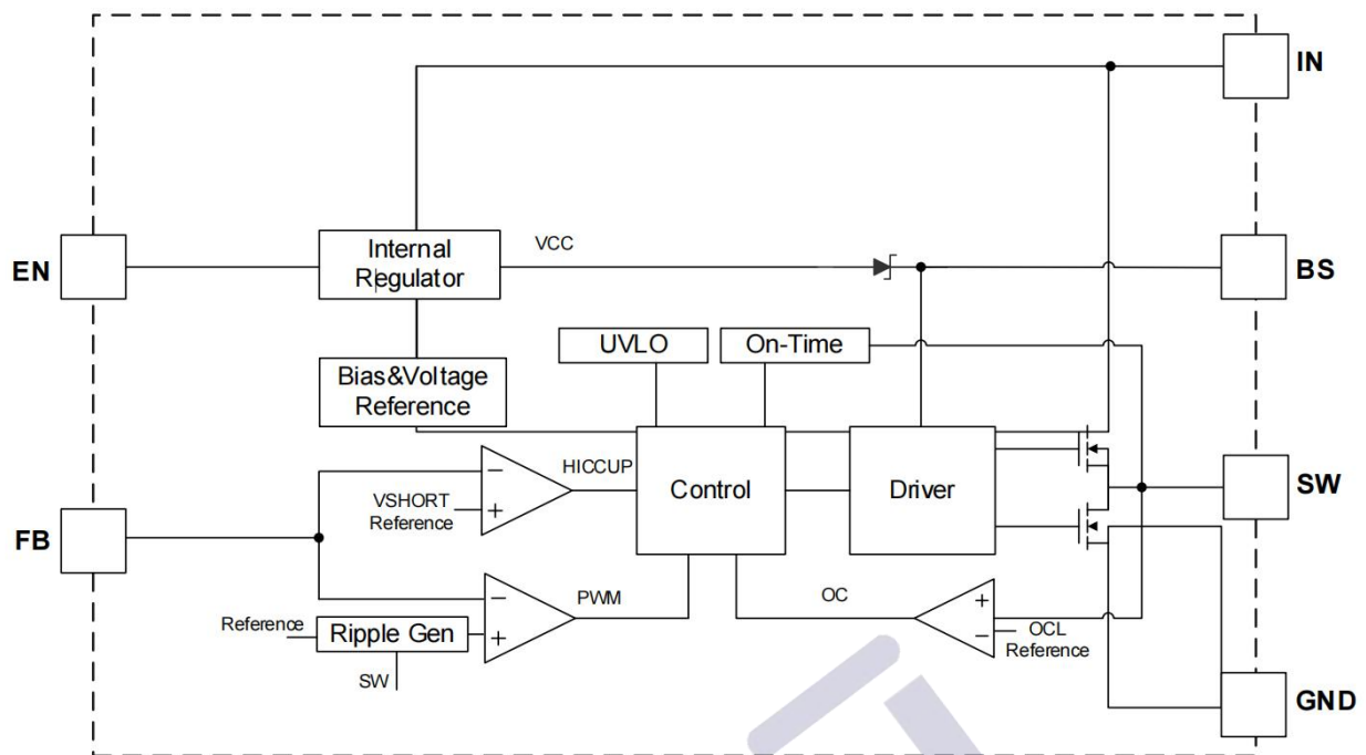
Block Diagram
