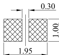
METAL MASK T=0.08 TOLERANCE: ±0.05MM (FOR REFERENCE ONLY)
