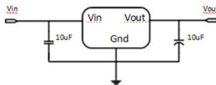
Application circuit of LM1117MPX-xx/NOPB fixed version
