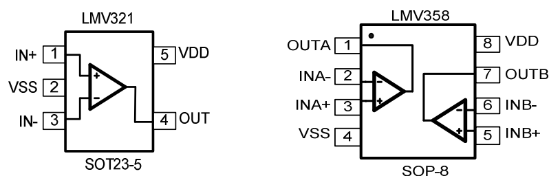
Figure 1. Pin Assignment Diagram
