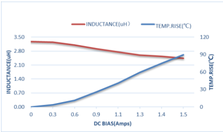
ZEP IM160808T3R3MLF
