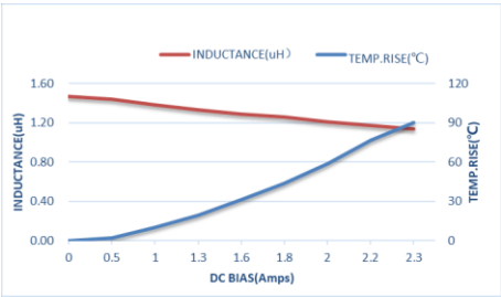
ZEP IM160808T1R5MLF
