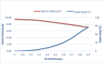
ZEP IM160808T100MLF
