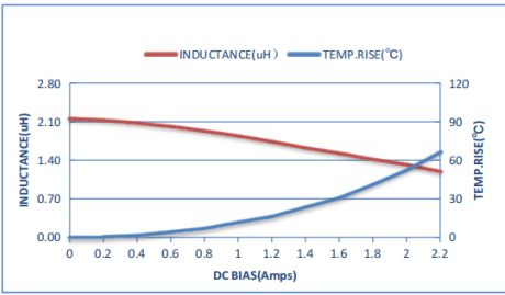
ZEP IM160808T2R2MLF
