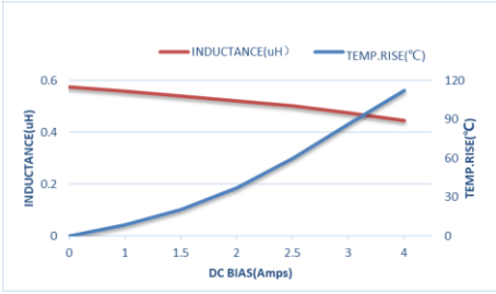
ZEP IM160808TR56MLF
