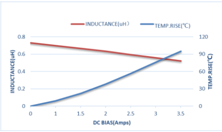
ZEP IM160808TR68MLF
