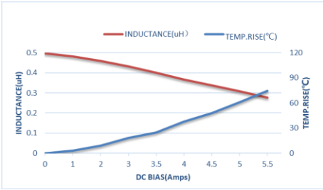
ZEP IM160808TR47MLF
