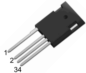
TO-247-4L (TO-247-4) Package
