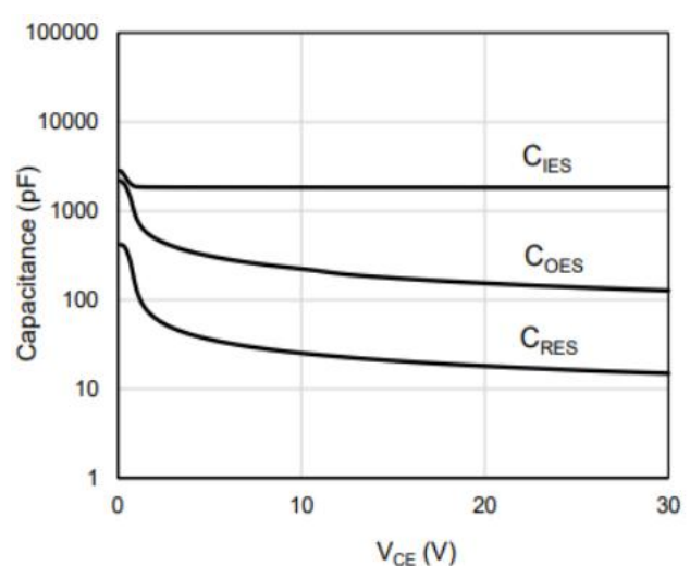
Fig.6 Typical capacitance
