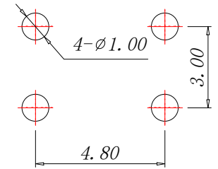
PCB.WELDING DRAWING
