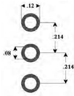
TO-247
