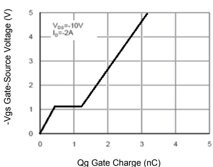
Figure 11 Gate Charge
