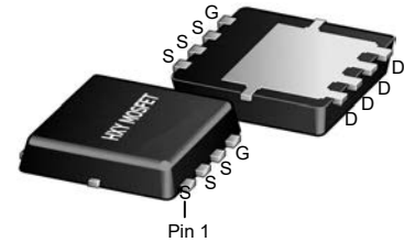
DFN5X6-8L (TDSON-8(5.9x5.2))
