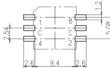
P.C.B DIMENSION (Top View)
