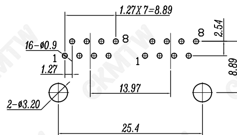
PC Board Layout Top View
