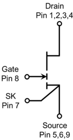
DFN8X8 (DFN-8(8X8))
