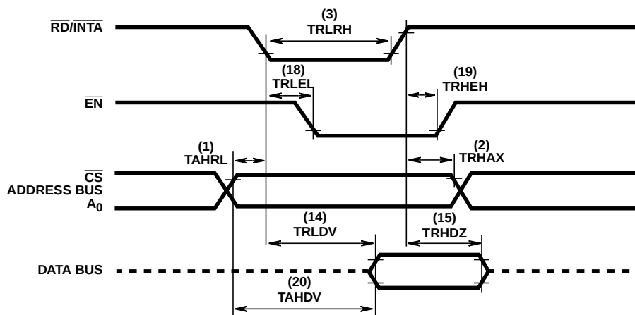
FIGURE 13. READ/INTA
