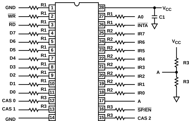
MR82C59A CLCC
