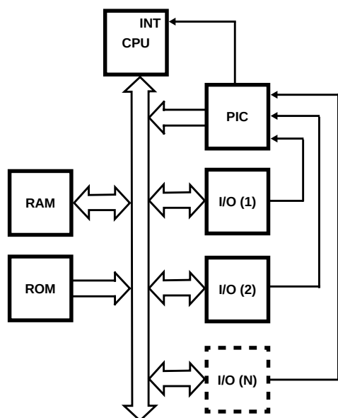
FIGURE 3. INTERRUPT METHOD
