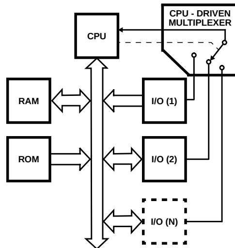
FIGURE 2. POLLED METHOD
