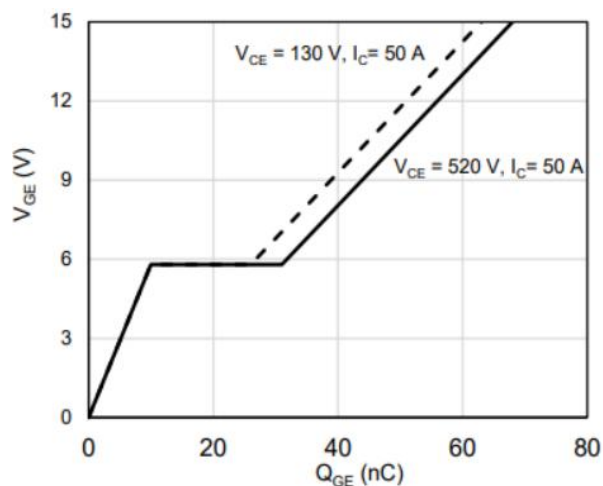
Fig.5 Gate charge
