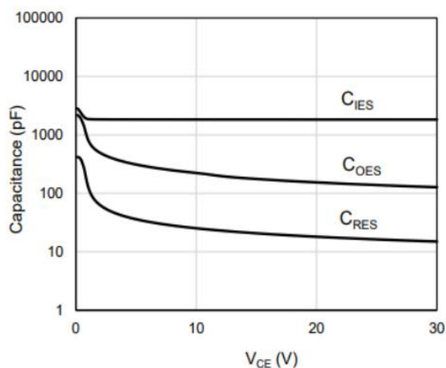
Fig.6 Typical capacitance
