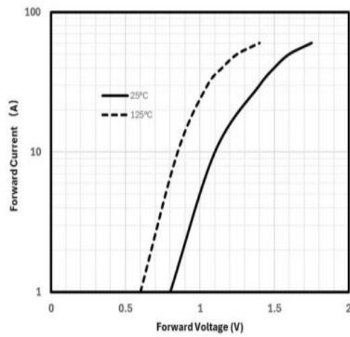
Fig.8 Typical diode VF vs. IF Characteristics
