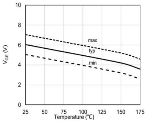
Fig.9 Threshold voltage vs. Junction temperature
