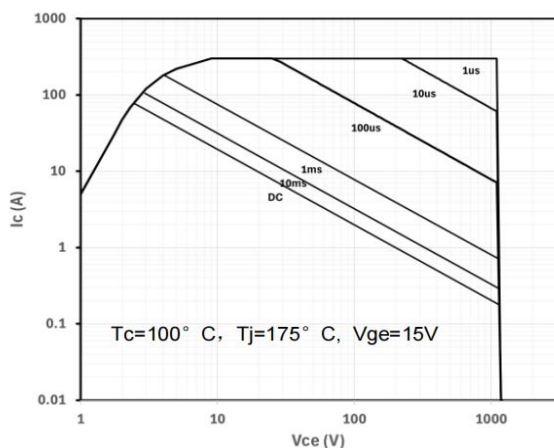
Fig.3 Forward Bias Safe Operating Area
