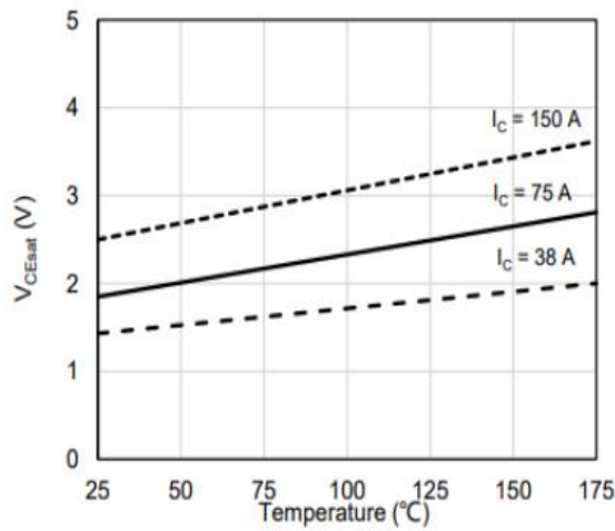
Fig.7 Vcesat vs. Junction Temperature
