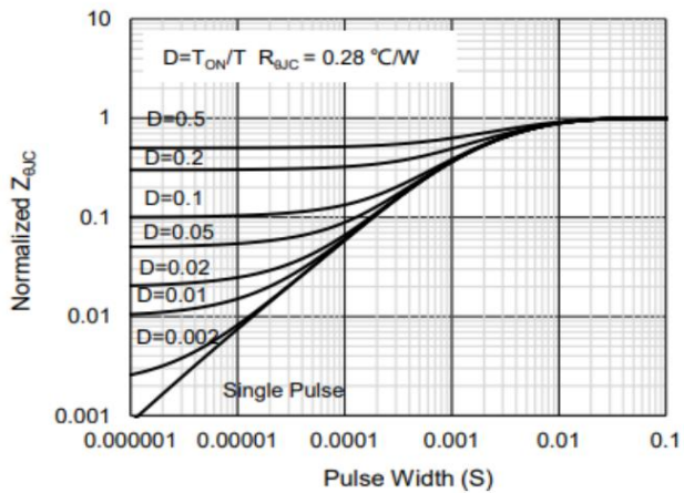
Fig.13 Transient Thermal Impedance Diode
