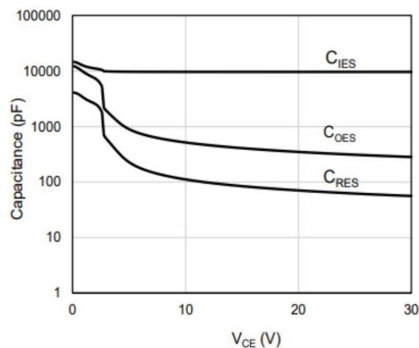
Fig.6 Typical capacitance
