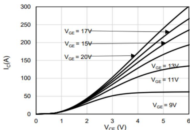
Fig.2 Typical Output characteristics (175°C)
