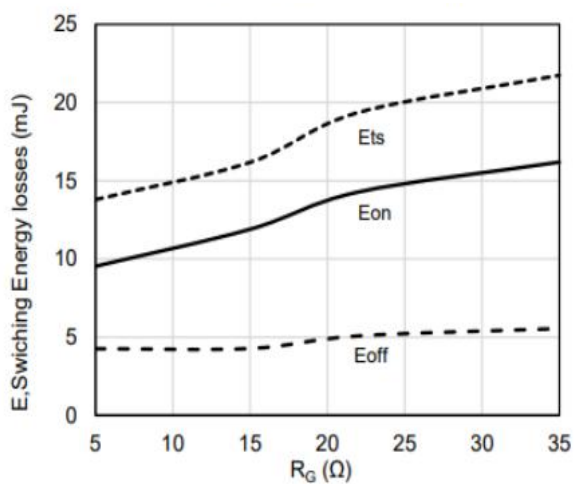
Fig.11 Switching Energy Loss vs. R G
