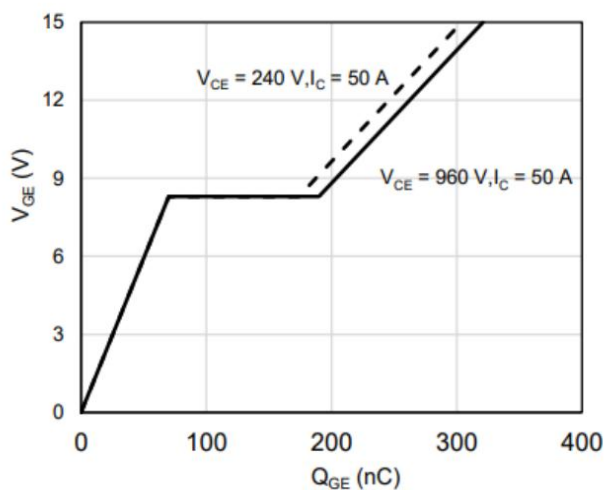
Fig.5 Gate charge
