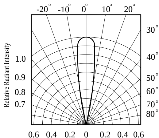
Fig.5 Relative Radiant Intensity vs. Angular Displacement
