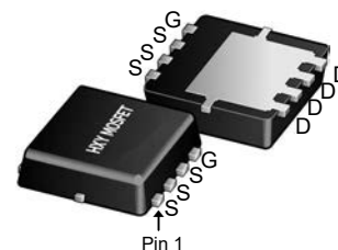
DFN3X3-8L (HSMT-8(3.2x3))
