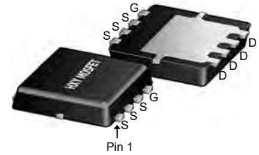
DFN5X6-8L (VSONP-8(5x6))
