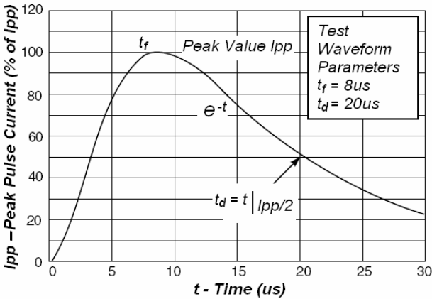
Fig1. Pulse Waveform
