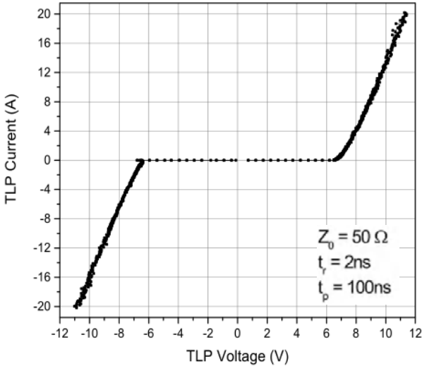
Fig2.TLP Measurement
