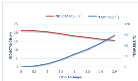
ZET-CORE-404020ST220MGCA
