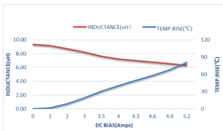
ZET-CORE-404020ST100MGCA
