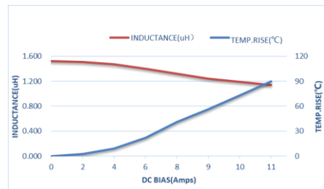
ZET-CORE-404020ST1R5MGCA
