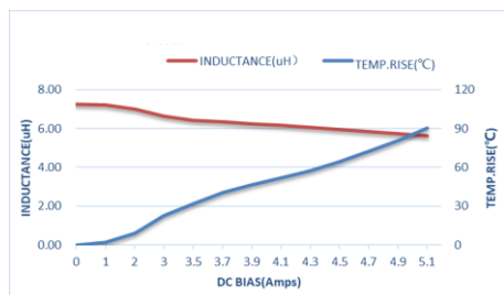
ZET-CORE-404020ST6R8MGCA
