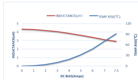
ZET-CORE-404020ST4R7MGCA
