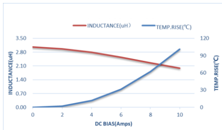
ZET-CORE-404020ST3R3MGCA
