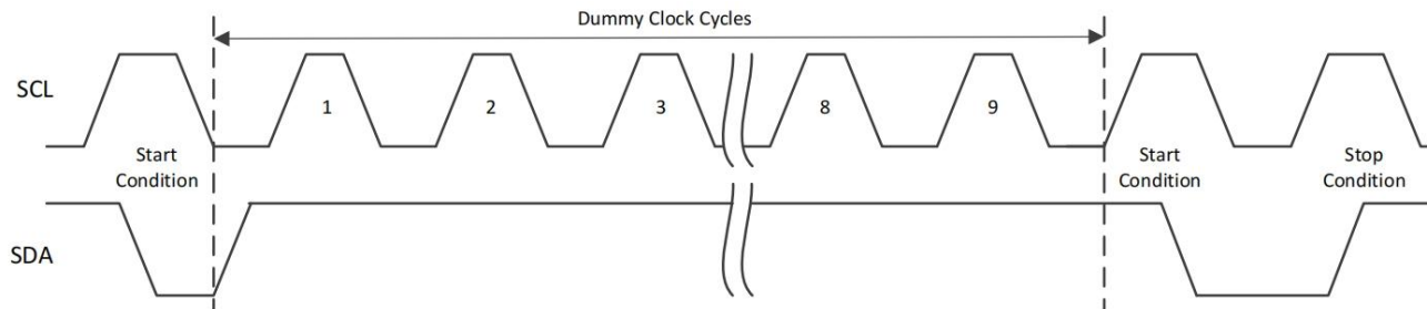
Figure 3–2 2-wire Software Reset
