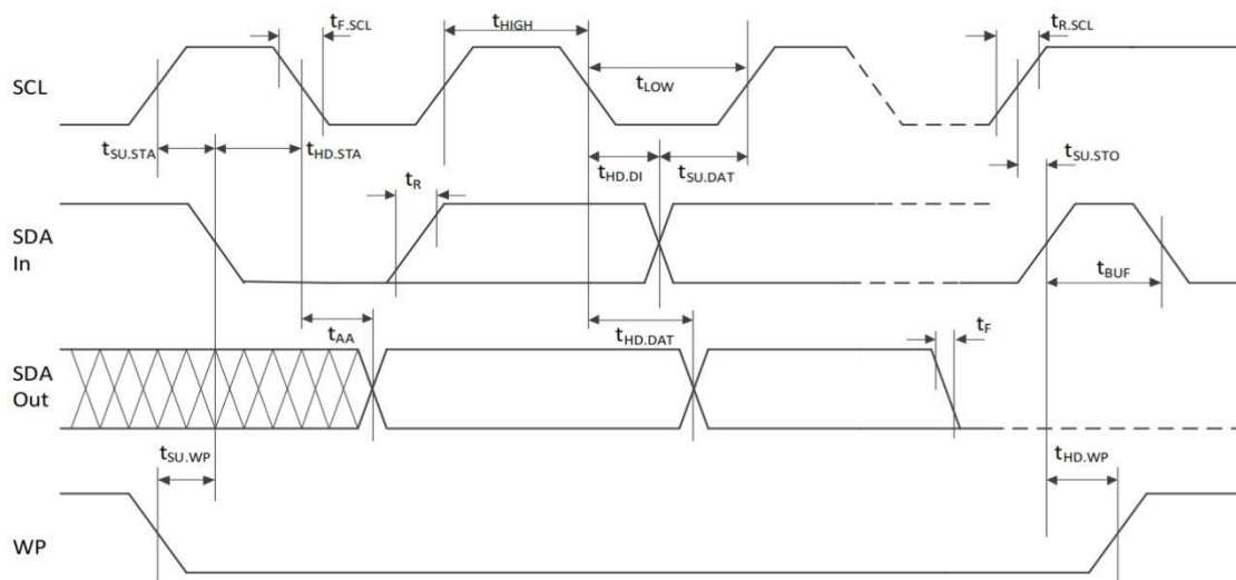
Figure 6–1 Bus Timing
